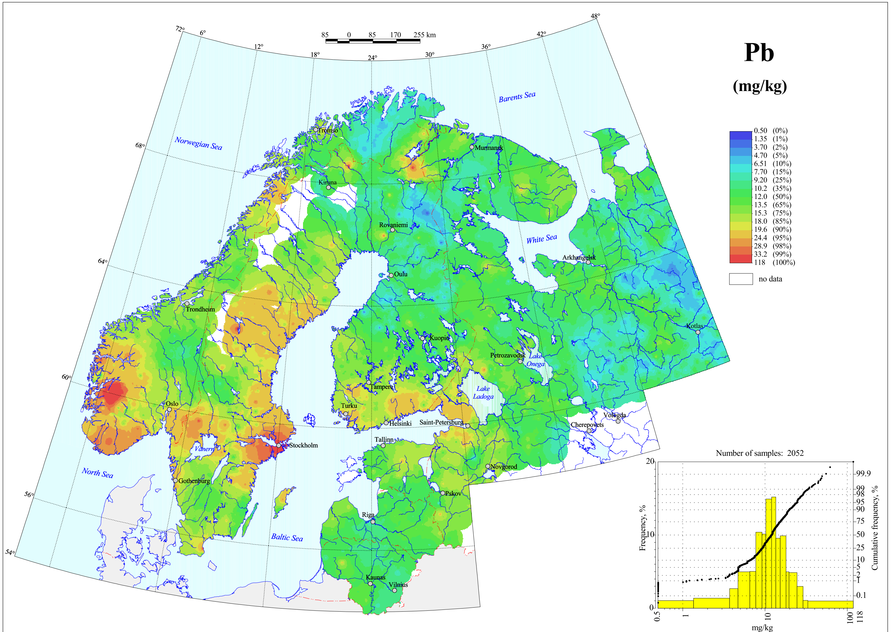
Lead in C-horizon, Grain Size <2 mm, Total Content
